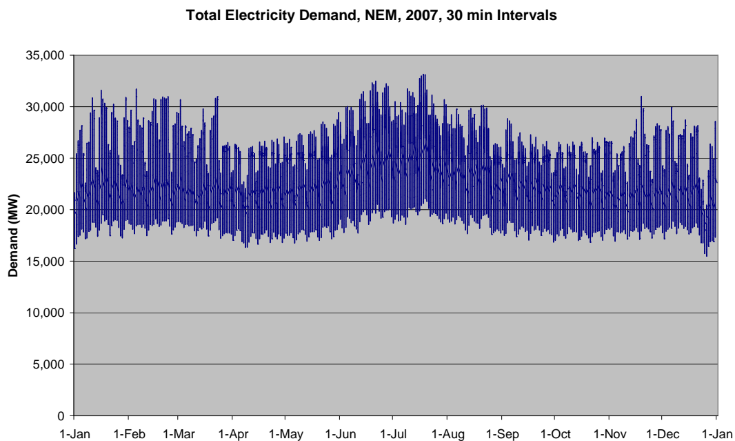
Figure 1 - the total electricity demand at 30 minute intervals throughout 2007. The peak occurs in July and shows we need 33,000 MW of generating capacity to meet the peak demand. (This is equivalent to the generating capacity of twenty-two Tumut 3 Power Stations 4 ). The base load 5 is about 18,000 MW for most of the year and about 20,000 MW in July.
